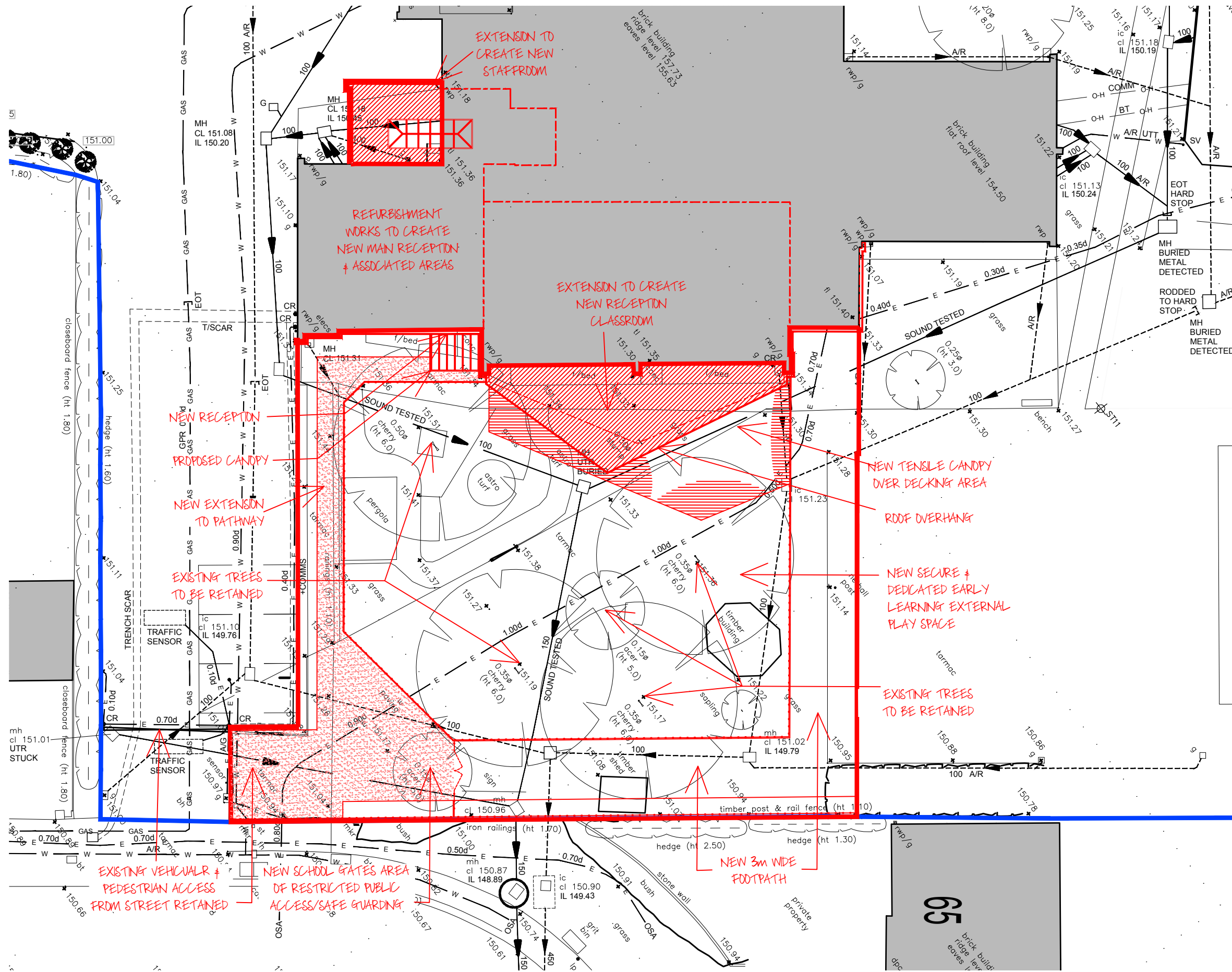
PROPOSED SITE LAYOUT 1:200
