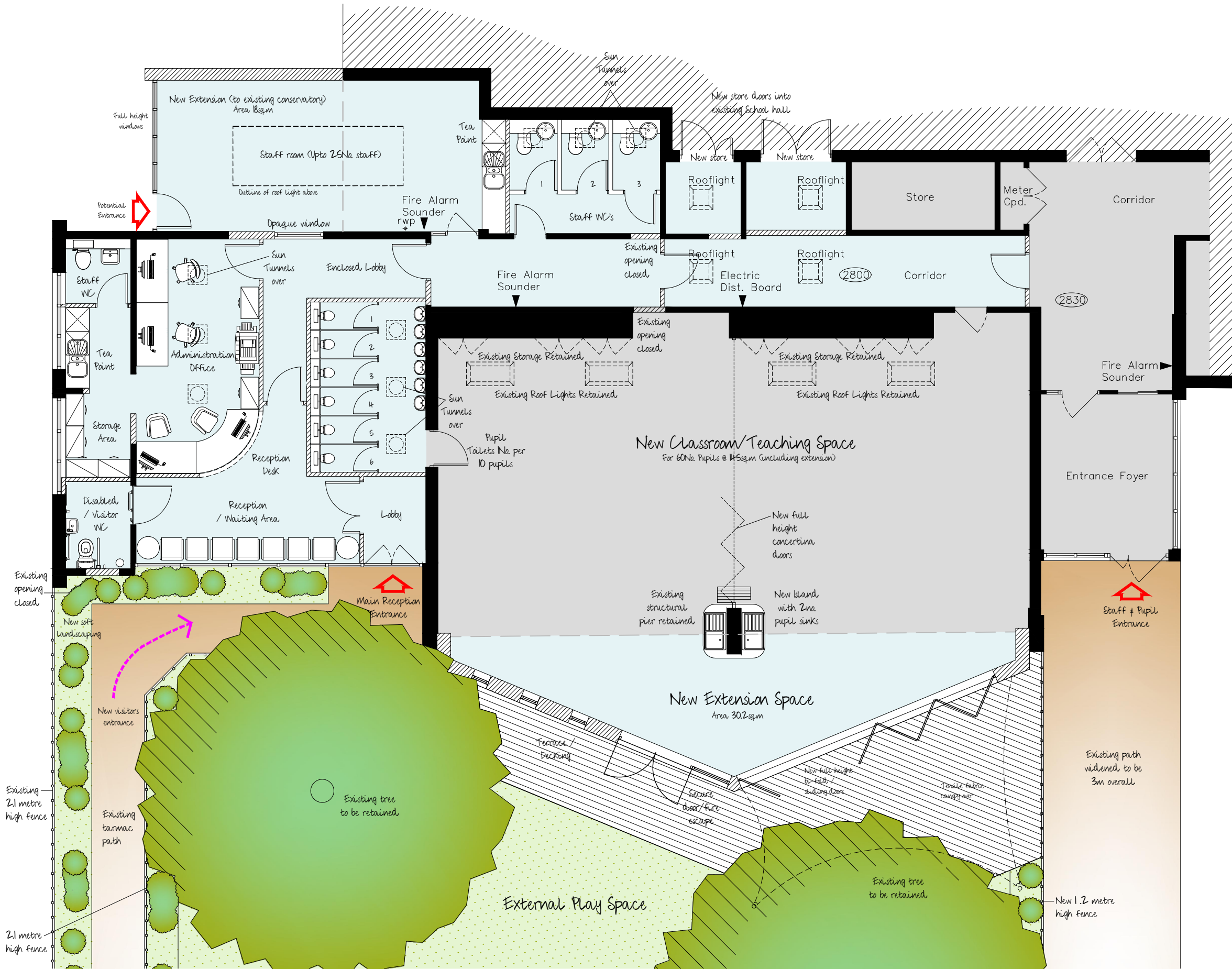
CONCEPTUAL FLOOR PLAN 1:100
